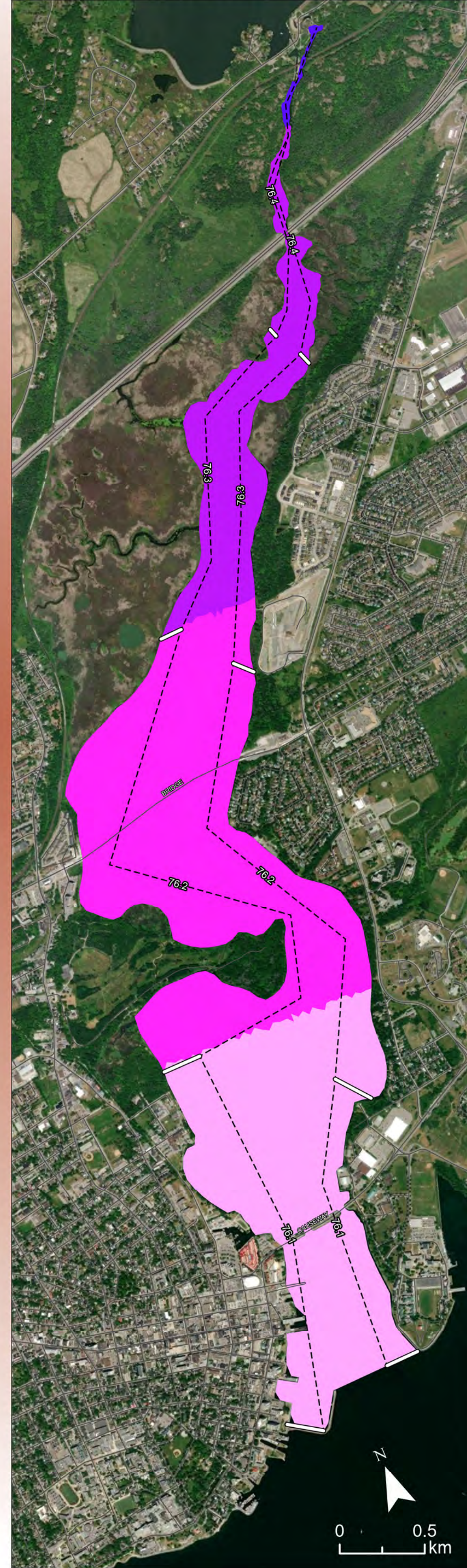
Run 1: Historical 100-yr flood level (76.09 m, IGLD'85 at Kingston). 100-year winds from 180°
