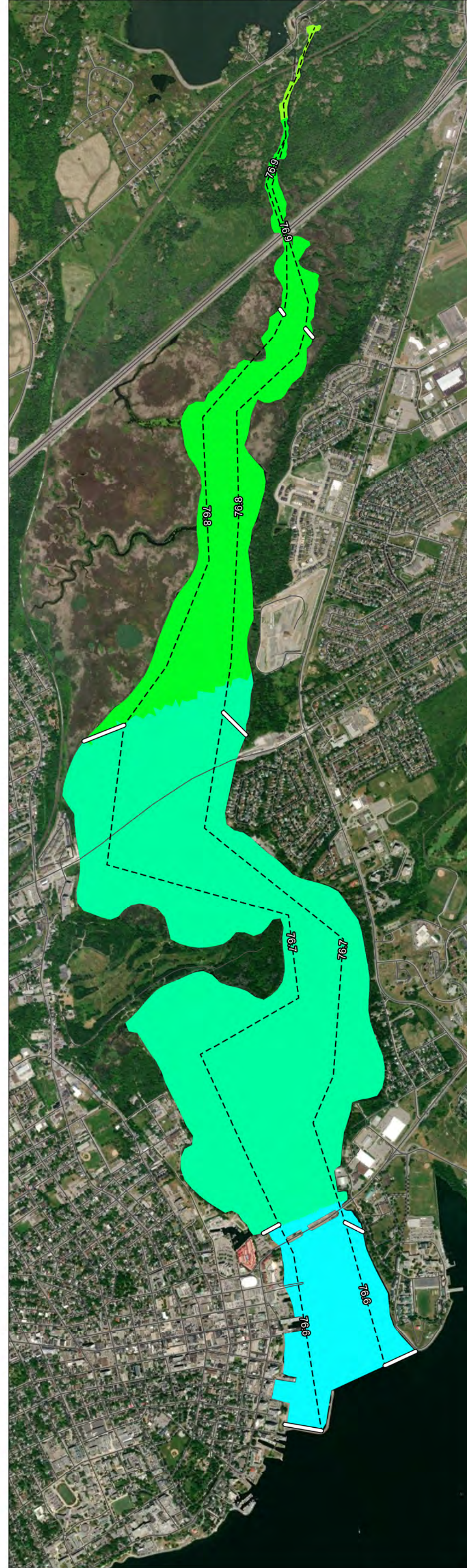
Run 3: Climate Change 100-yr flood level (76.62 m, IGLD'85 at Kingston). 100-year winds from 180°
